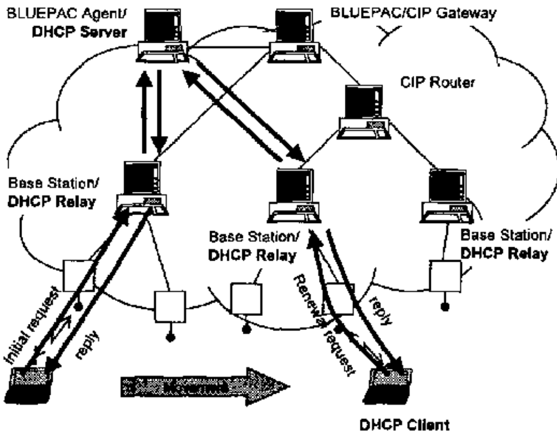
Figure 4: DHCP relay process
